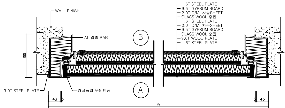
HORIZONTAL SECTION SCALE:1/2
